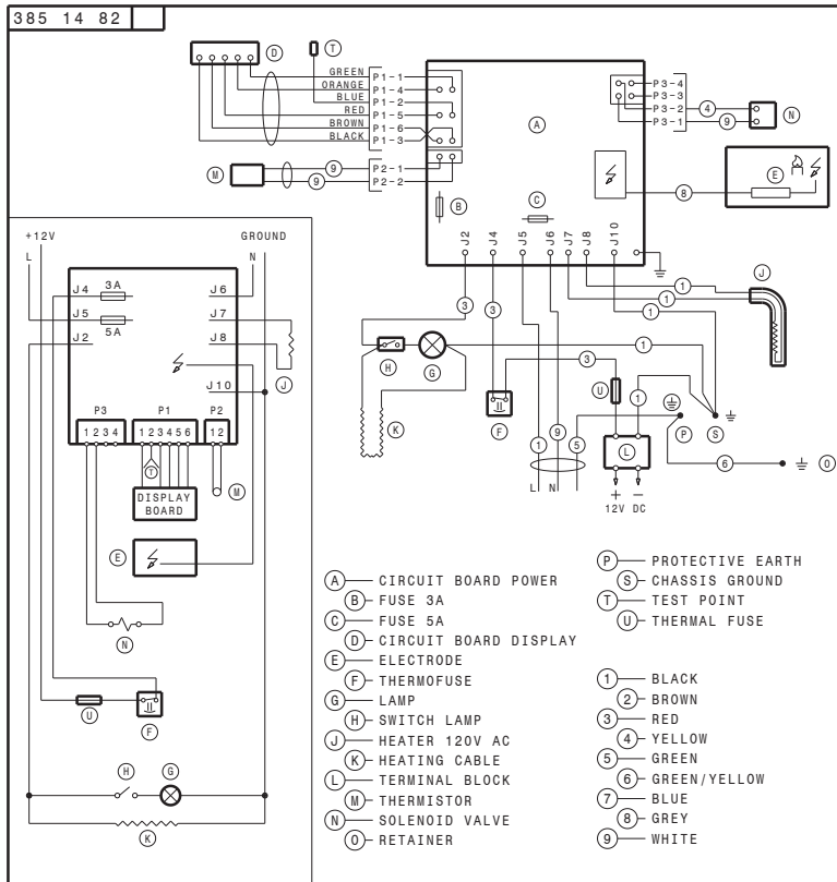
DM2652, DM2662, DM2852 & DM2862 (No Fan) With and Without Ice Maker
