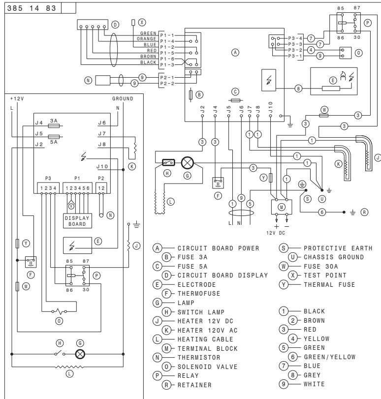
DM2663 (No Fan) Without Ice Maker
