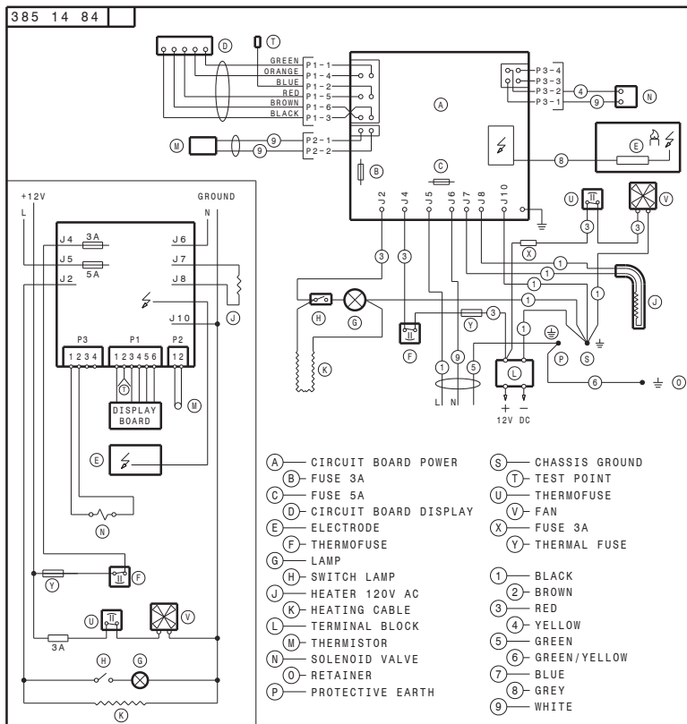
DM2652, DM2662, DM2852 & DM2862 (One Fan) With and Without Ice Maker
